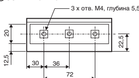
◎ SGLFW-20A120A□□
